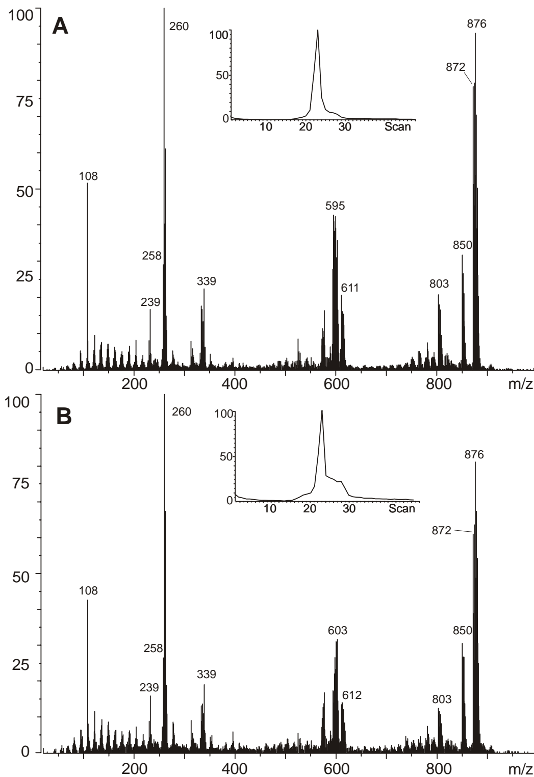
Figure 5. DTMS mass spectrum of (a) oil F, and (b) oil F300 (scan 23-25). Insert: Total Ion Chromatogram (TIC).
