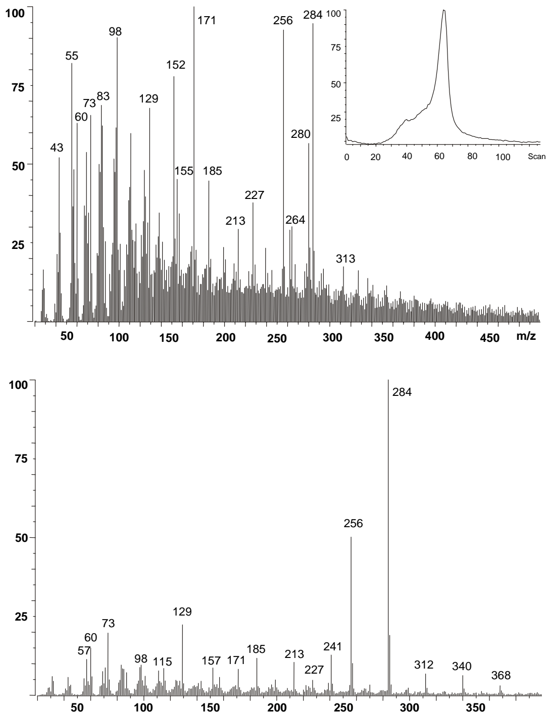
Figure 14. DTMS summation spectrum of 4-year-old dried linseed oil (Talens) (a) scan 56-64 Insert: TIC, and (b) scan 1-15.
