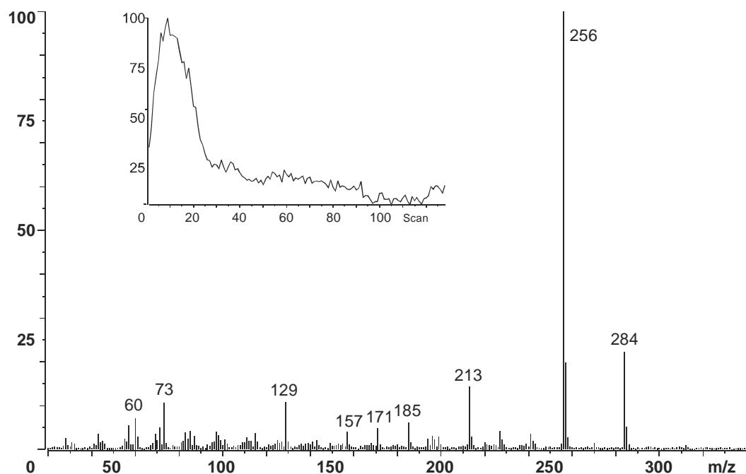
Figure 12. DTMS summation spectrum of scans 0-3- of crystals on surface of red paint panel #6 “Cricche, Crotche e Manico d’Unico”. Insert: TIC.
