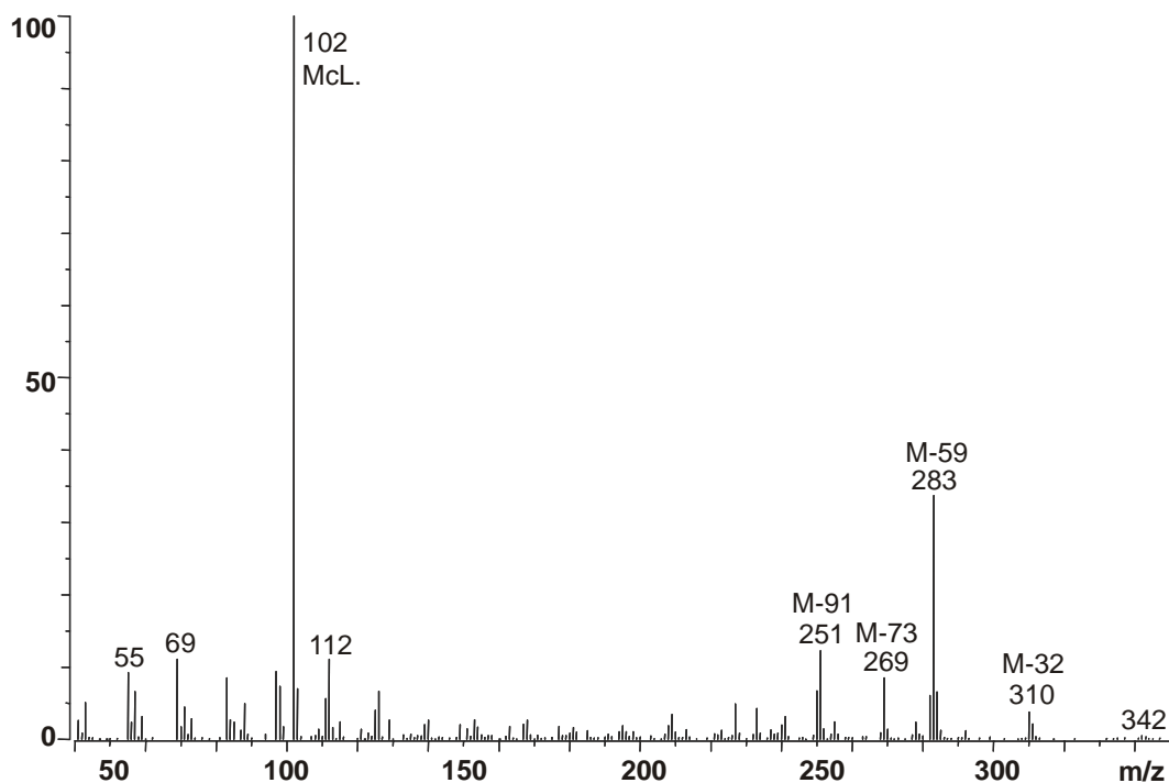
Figure 7. 70 eV EI mass spectrum of 2,2-dimethyl hexadecanedioic acid, dimethyl ester.
