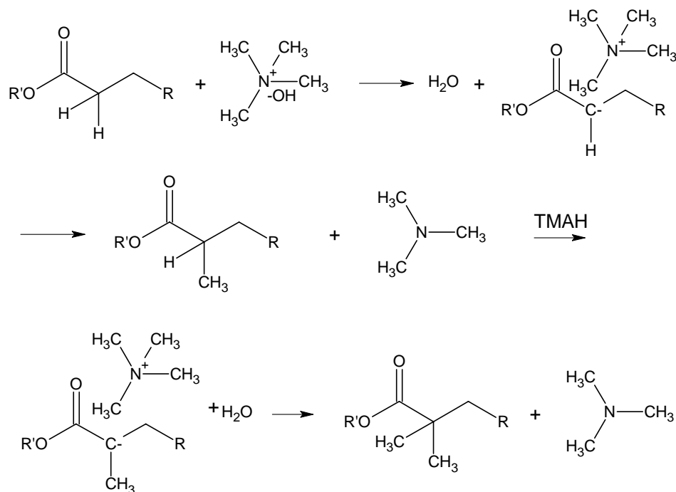
Scheme 2. Postulated mechanism of formation of \alpha - and \beta -methylated diacids.
