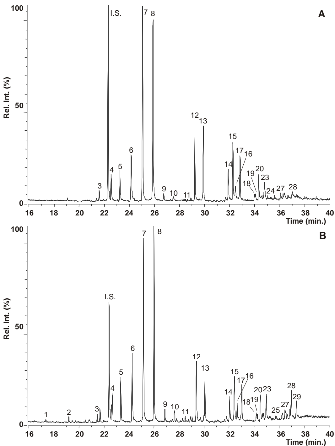
Figure 8a,b. Two TICs of a 27-year-old vine black pigmented oil film (CCI, Ottawa) after transesterification and trimethylsilylation derivatization. The numbers correspond to Table 2.
