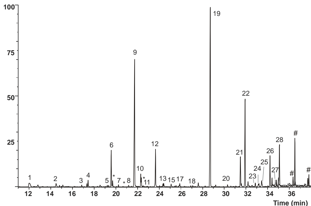
Figure 14. TIC of cobalt blue paint on panel #6 of “Cricche, Cricche e Manico d’Unico”, obtained by Cu-Py-TMAH-GC/MS analysis. Peaks labelled * are identified as dimethyl esters of phthalic acids,. Temperature program: 50(2)-6-320.
