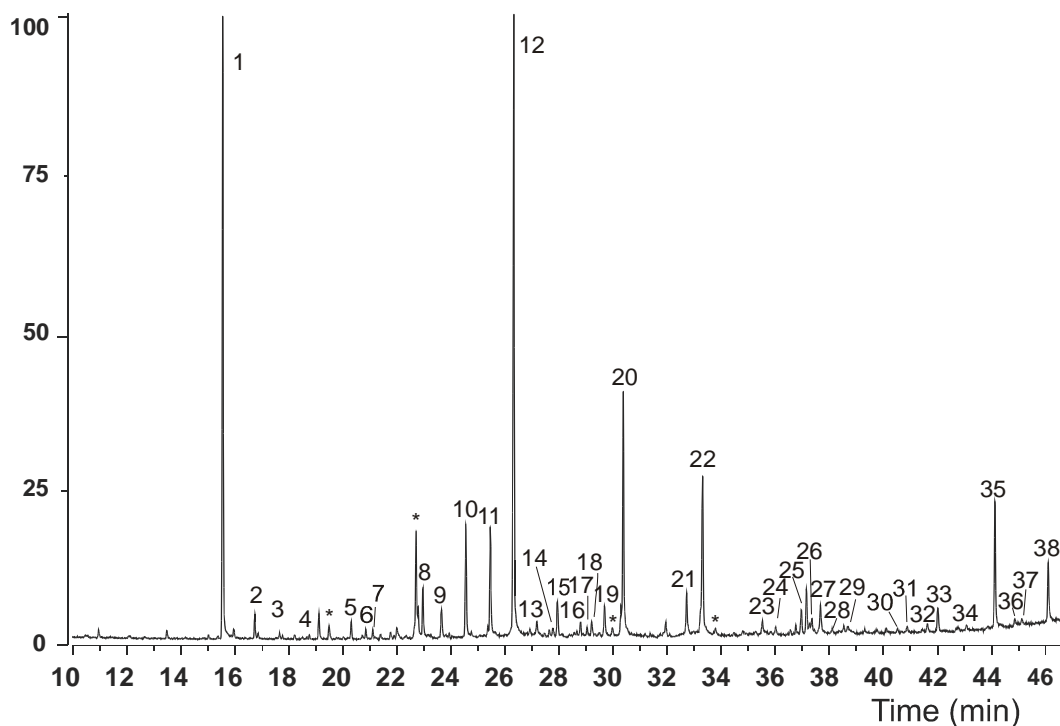
Figure 3. Total ion chromatogram of cream-coloured paint of OL.NA after transesterification and trimethyl silylation derivatisation in combination with GC/MS using an on-column injector. Temperature program: 50(2)-6-320. Peak numbers correspond to Table 3. Peaks labelled * are identified as polysiloxanes.
