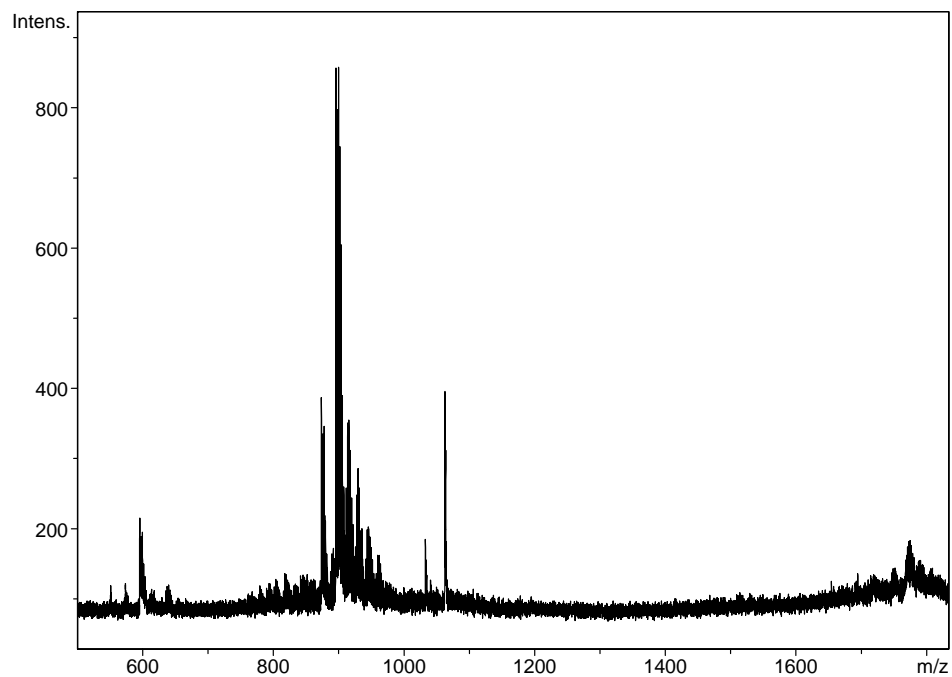
Figure 6. MALDI-TOF-MS spectrum of oil F300 (Reflectron mode)
