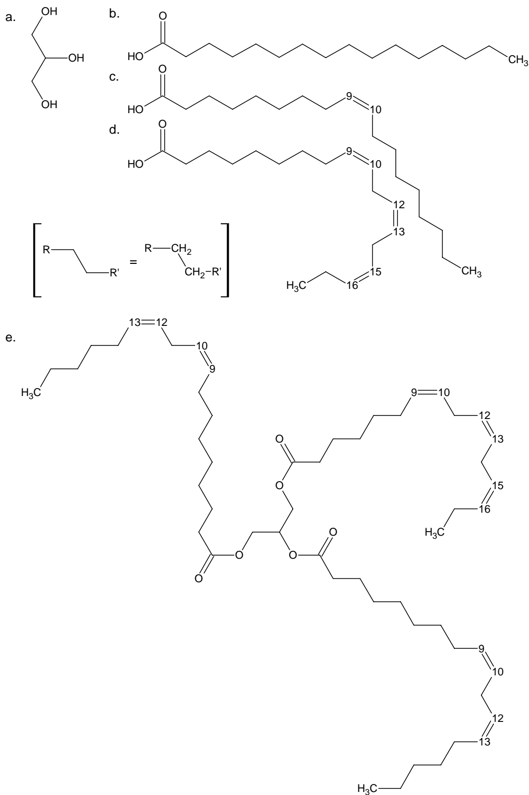
Figure 1. Constituents of a drying oil. (a) glycerol; (b) palmitic acid (C16); (c) oleic acid (C18:1); (d) linolenic acid (C18:3), and (e) a triacylglycerol with C18:2-C18:3 fatty acid moieties (TAG).
