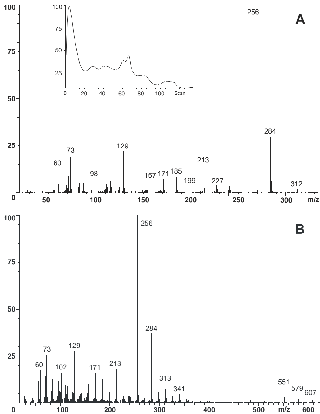
Figure 9 DTMS summation spectrum of crystals on surface of cobalt blue paint panel #6 “Cricche, Cricche e Manico d’Unico”, (a) scans 0-30, insert: TIC, and (b) scans 37-44
