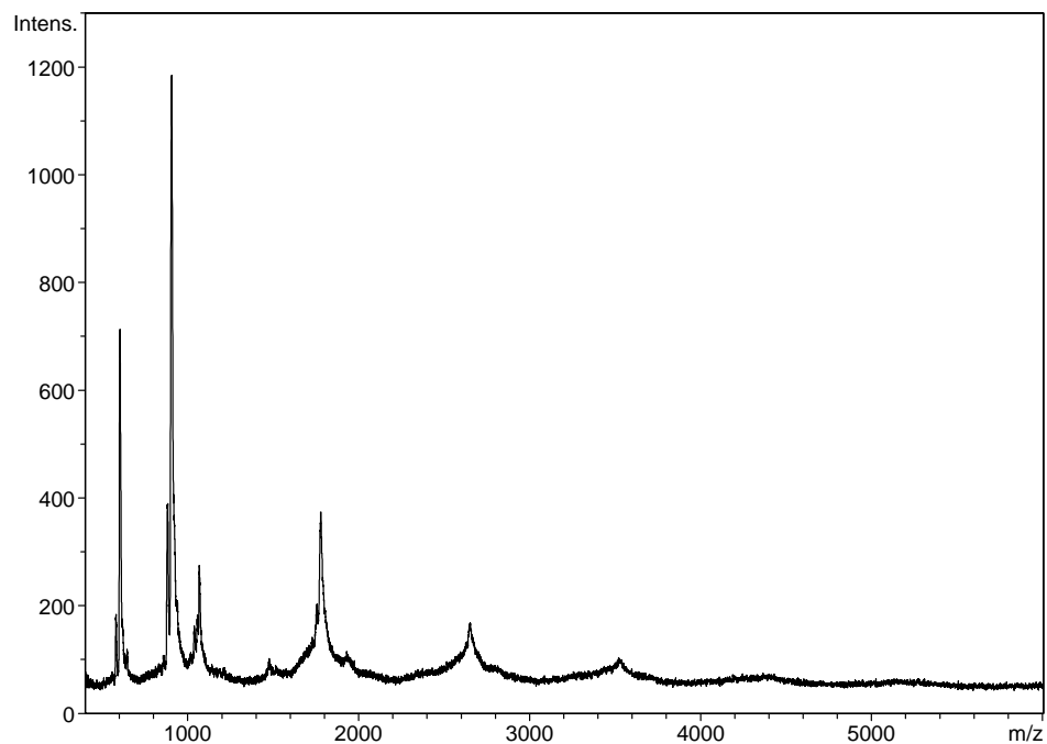
Figure 7. MALDI-TOF-MS spectrum of oil F300 (Linear mode).
